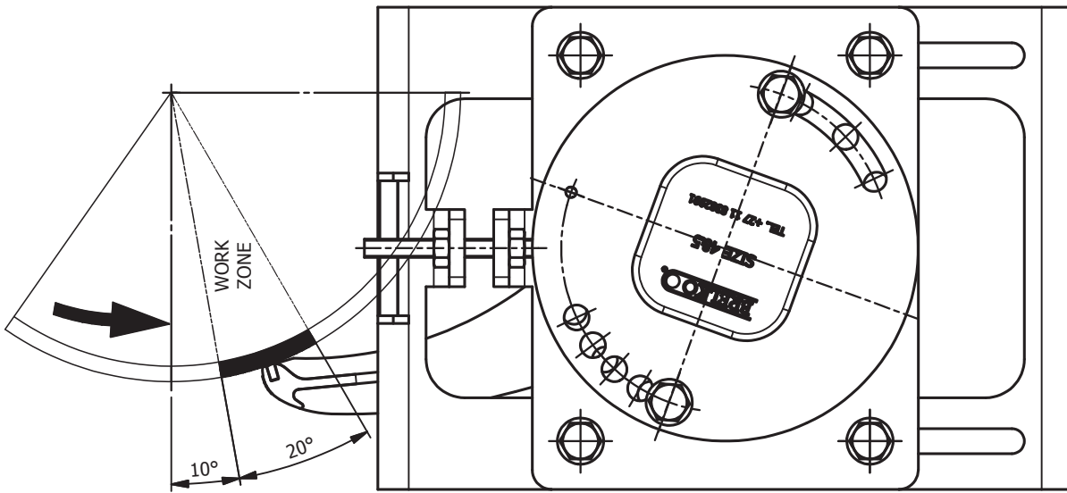
E951-TT TWIST TENSIONER MOUNTING
